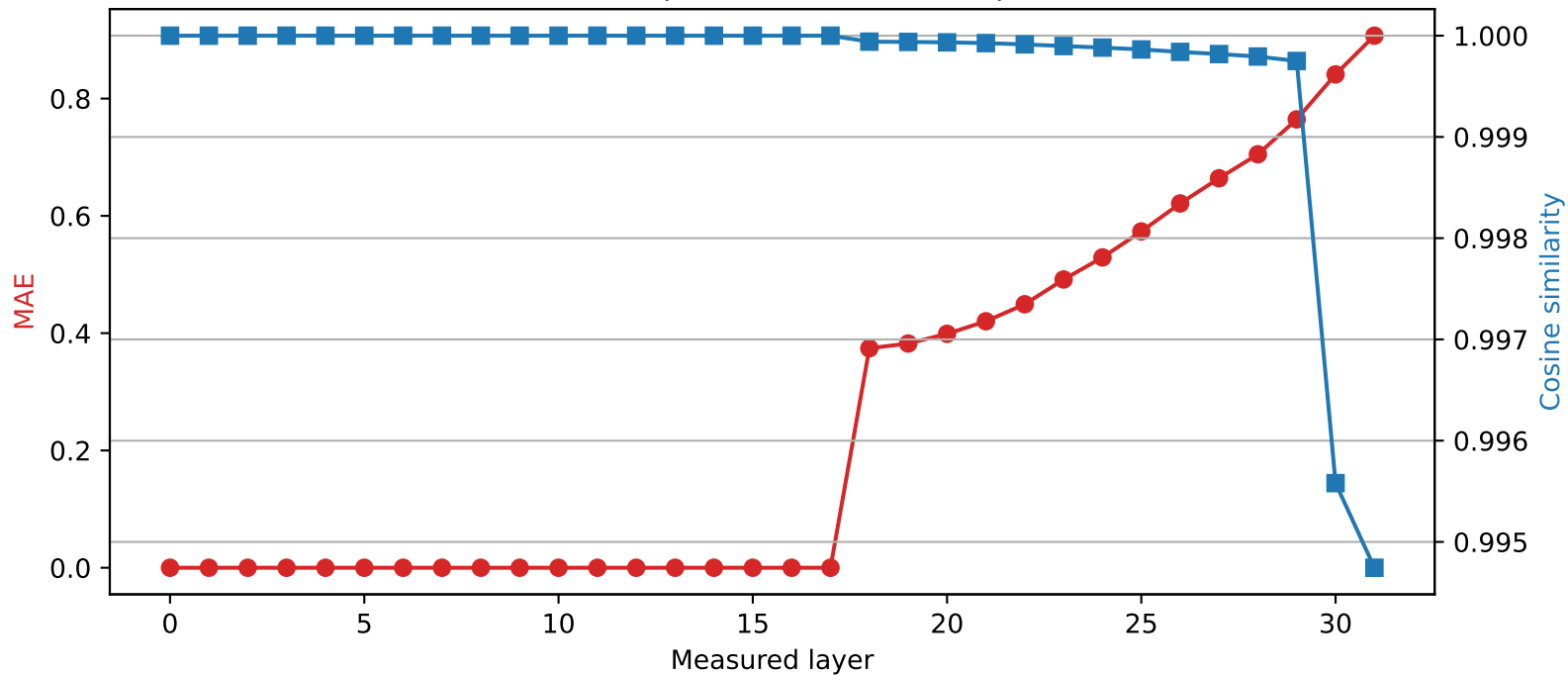
Phi-3-mini-4k-instruct | Quantized layer 17 | float16 \rightarrow int4
