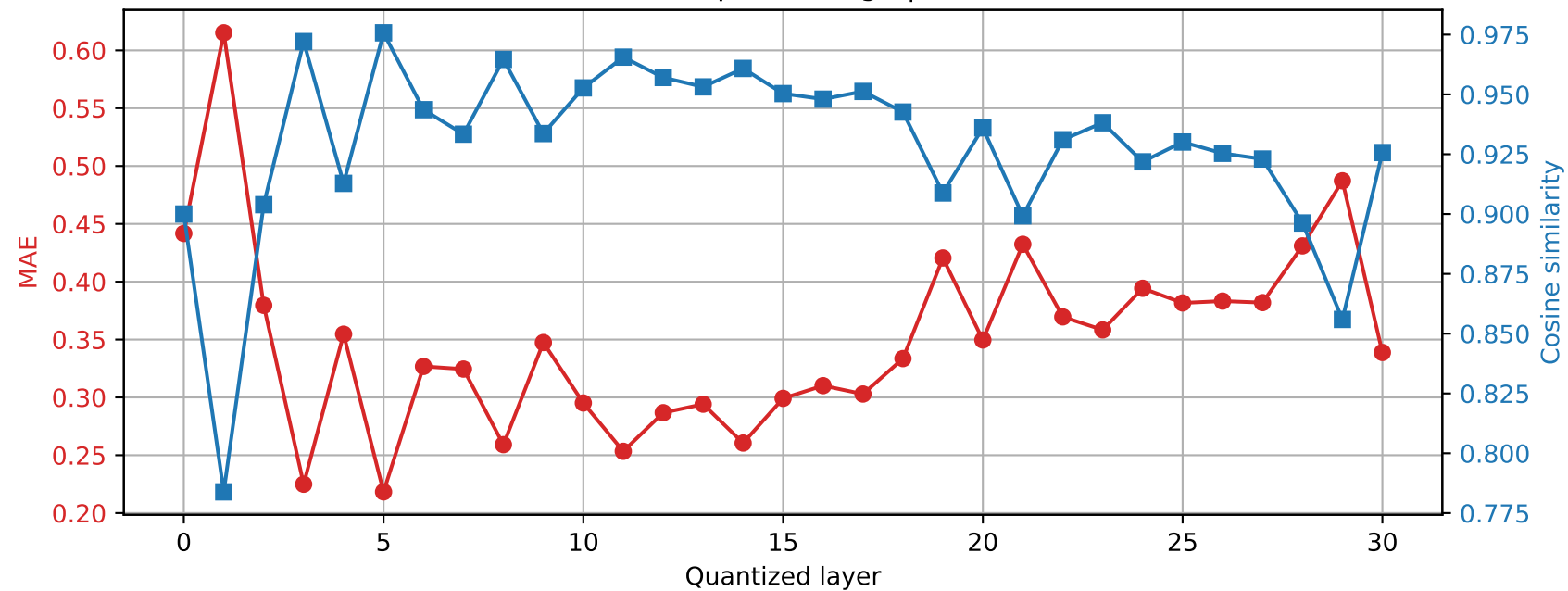
Phi-3-mini-4k-instruct | Prompt 1 Final RMSNorm output damage | float16 \rightarrow int4
