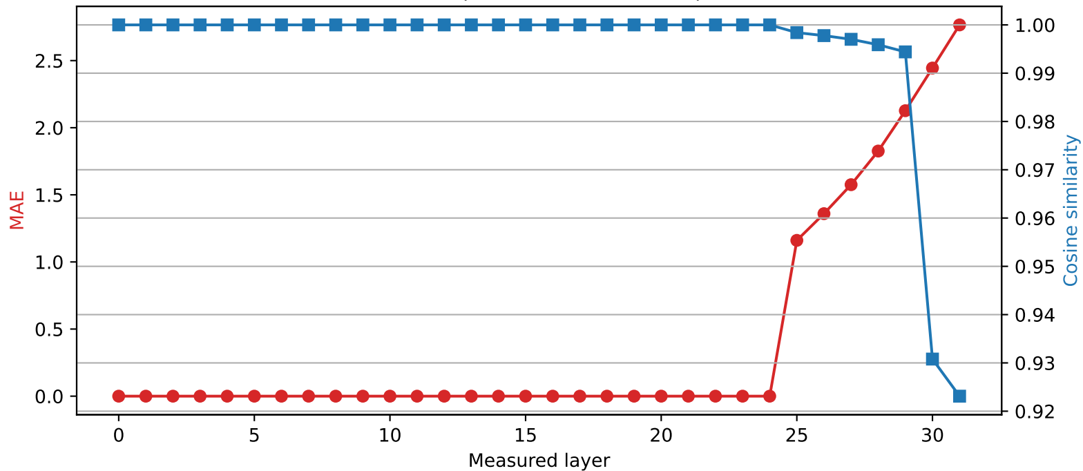
Phi-3-mini-4k-instruct | Quantized layer 24 | float16 \rightarrow int4
