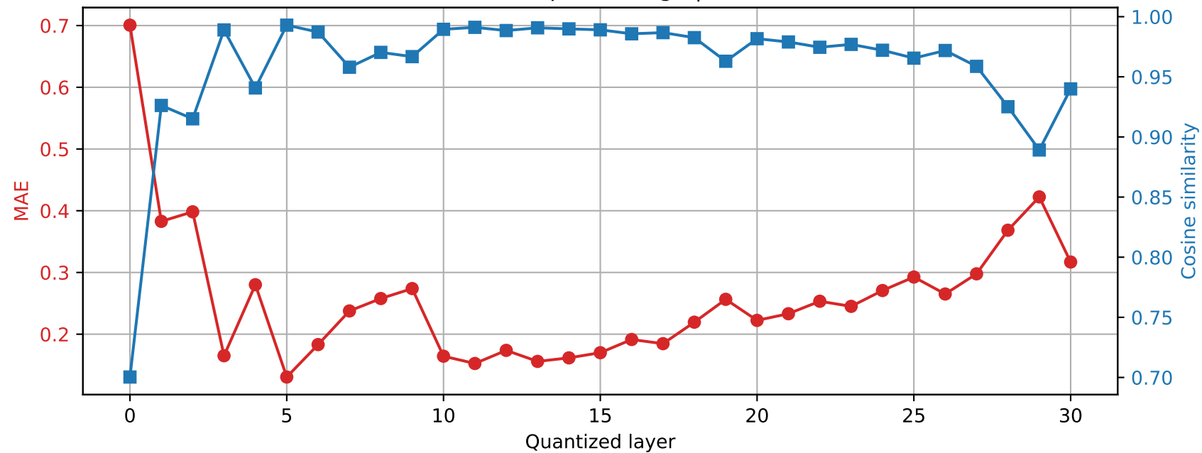
Phi-3-mini-4k-instruct | Prompt 2 Final RMSNorm output damage | float16 \rightarrow int4
