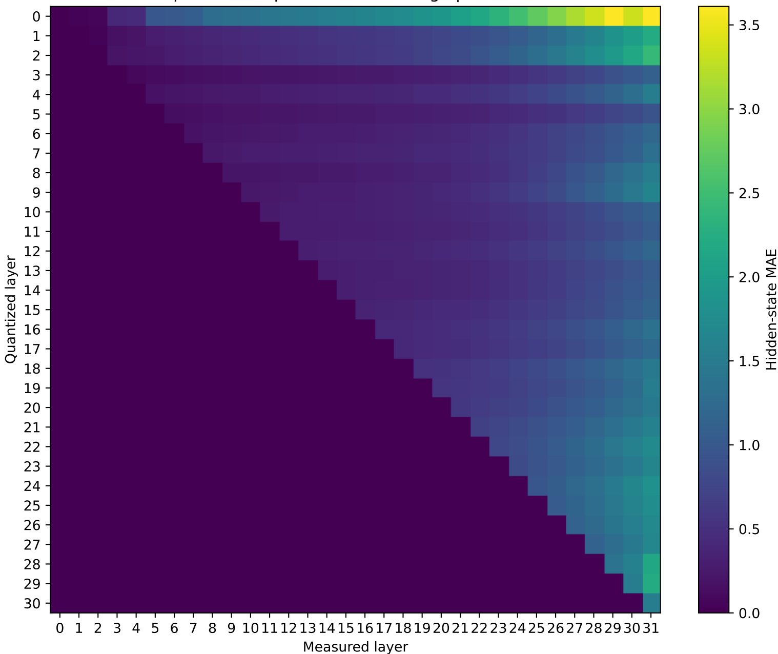
Phi-3-mini-4k-instruct Prompt 2: MAE representation damage | float16 \rightarrow int4
