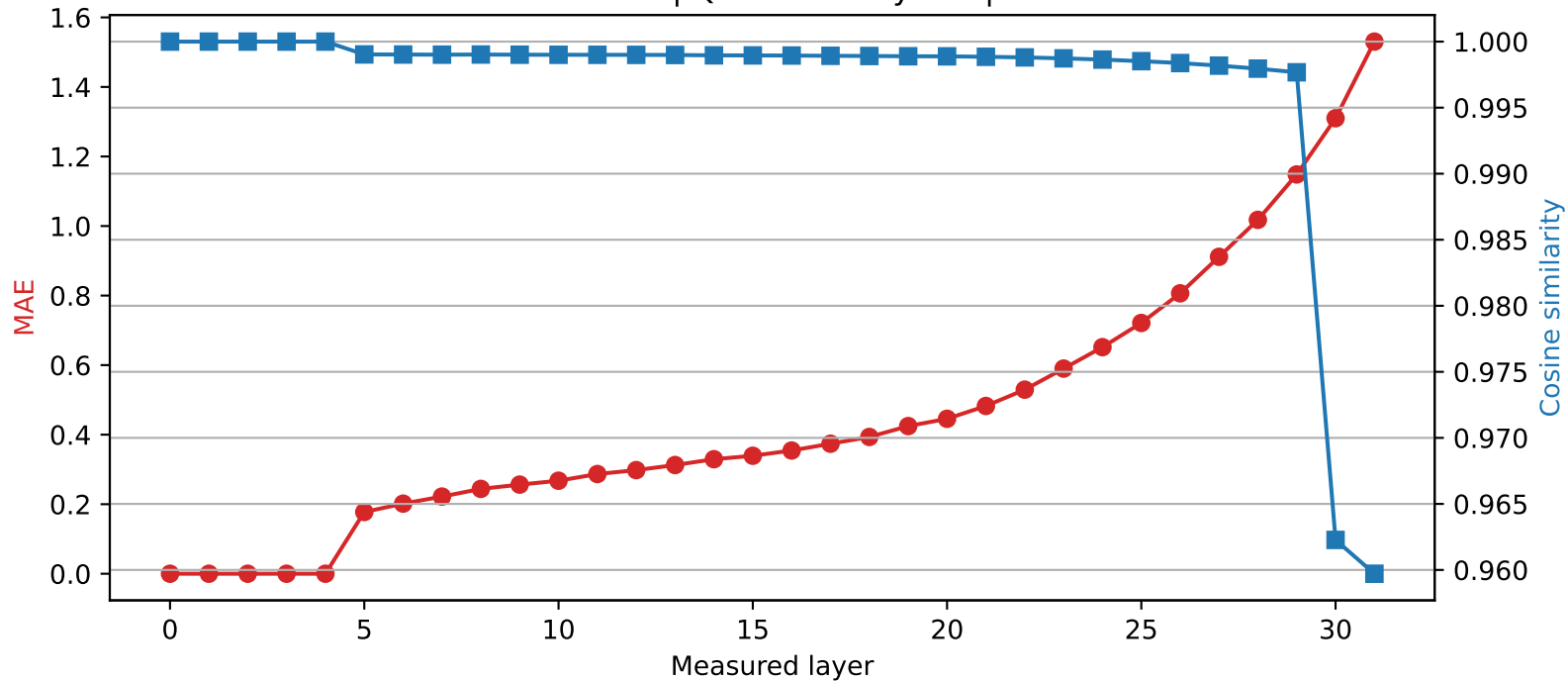
Phi-3-mini-4k-instruct | Quantized layer 4 | float16 \rightarrow int4
