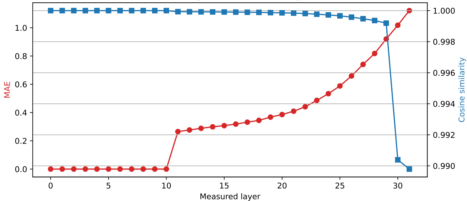
Phi-3-mini-4k-instruct | Quantized layer 10 | float16 \rightarrow int4
