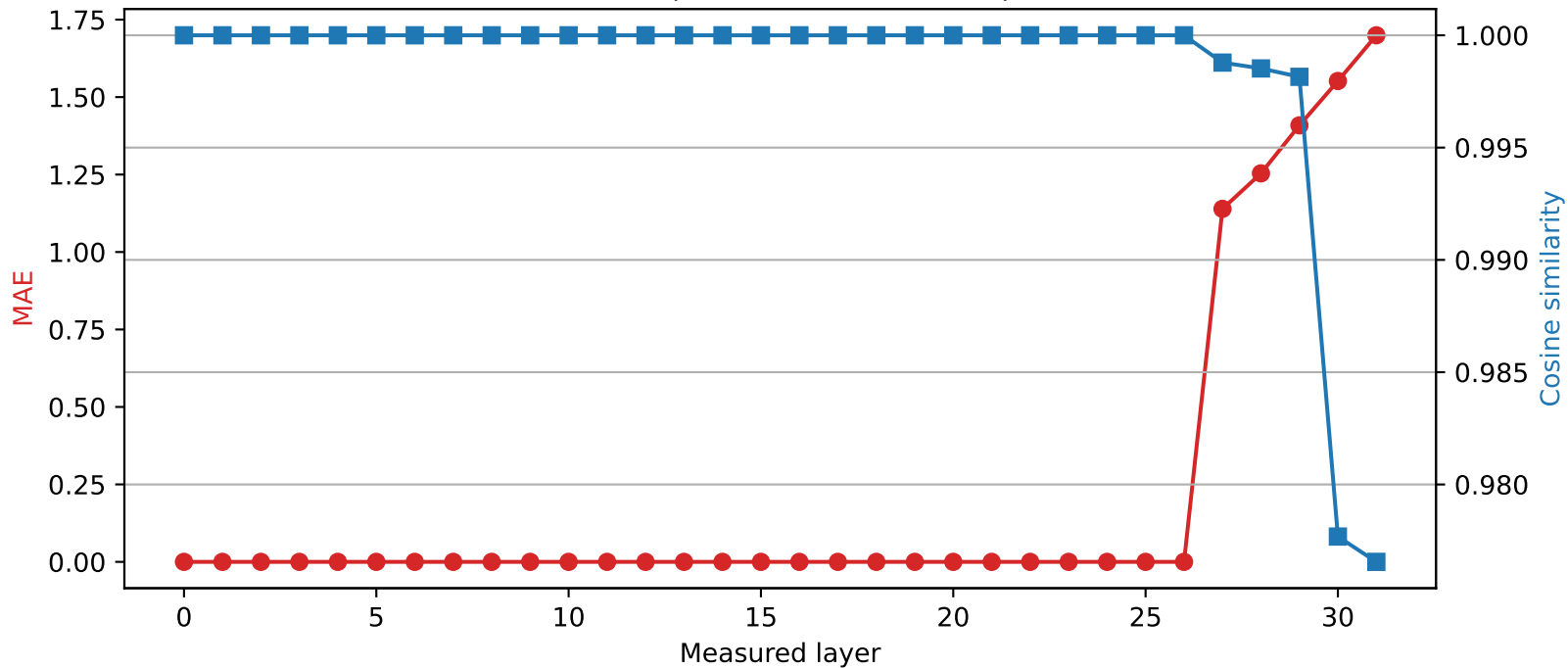
Phi-3-mini-4k-instruct | Quantized layer 26 | float16 \rightarrow int4
