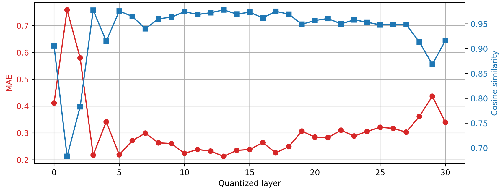
Phi-3-mini-4k-instruct | Prompt 3 Final RMSNorm output damage | float16 \rightarrow int4
