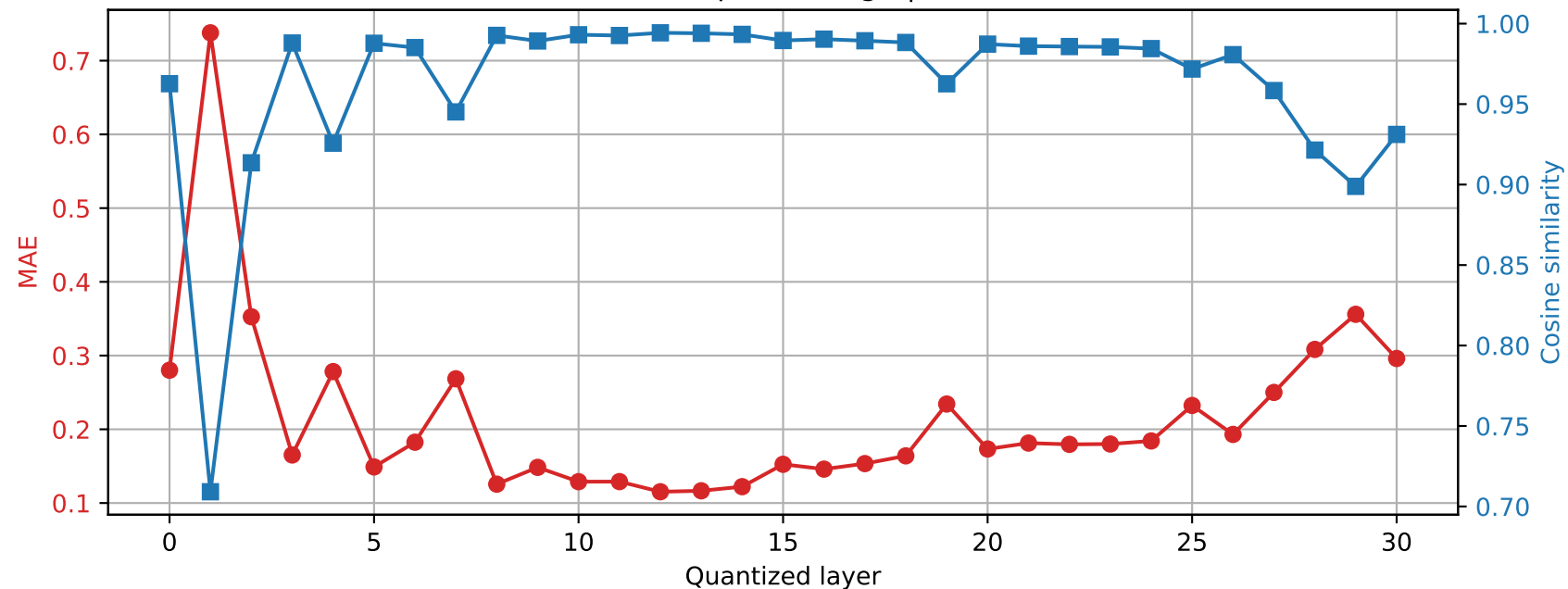
Phi-3-mini-4k-instruct | Prompt 4 Final RMSNorm output damage | float16 \rightarrow int4
