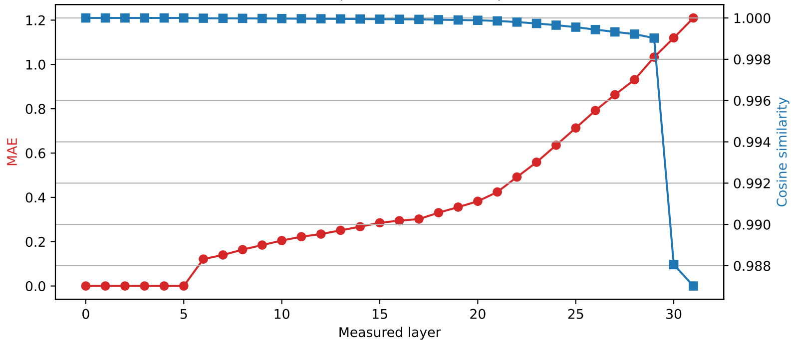
Phi-3-mini-4k-instruct | Quantized layer 5 | float16 \rightarrow int4
