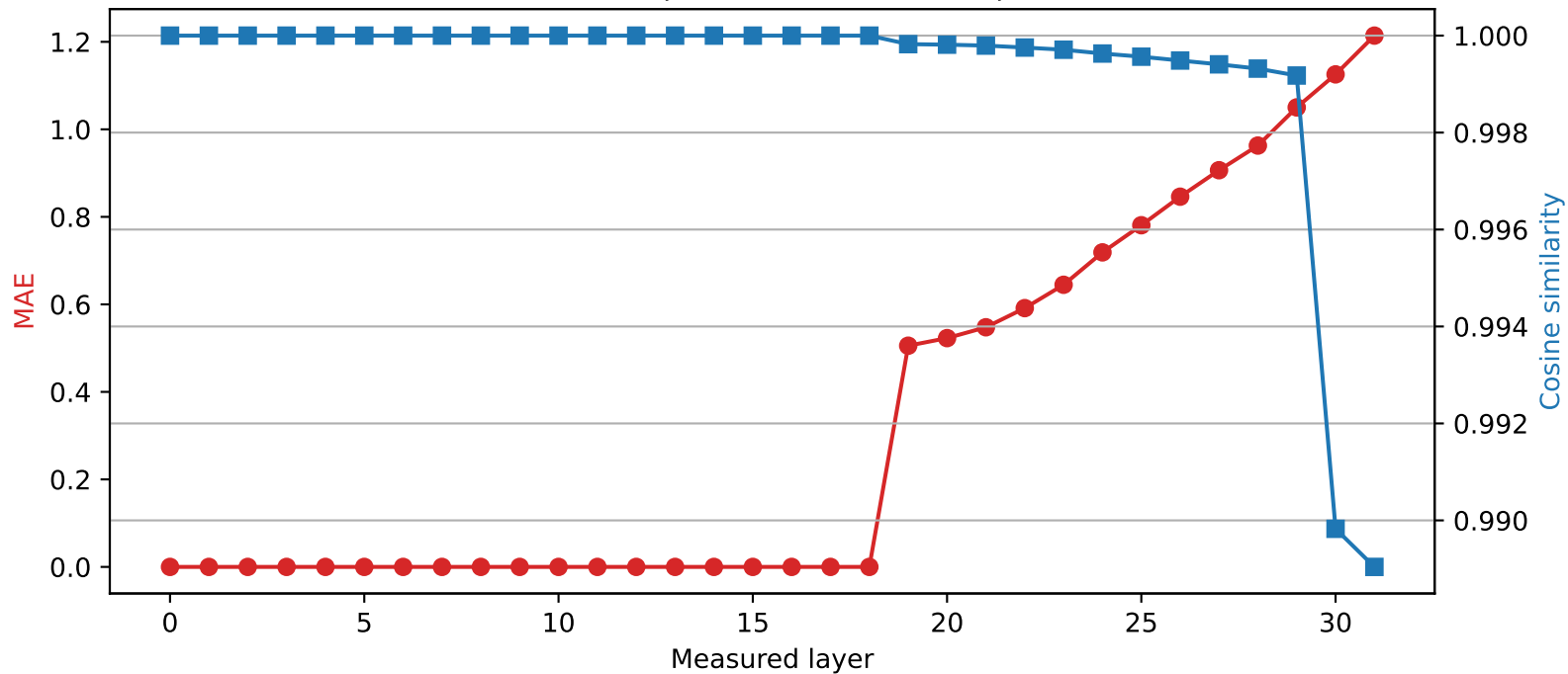
Phi-3-mini-4k-instruct | Quantized layer 18 | float16 \rightarrow int4
