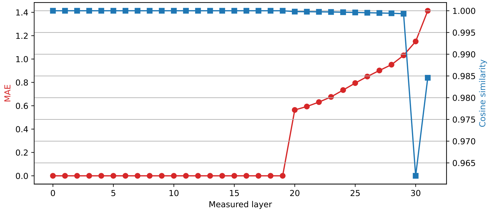
Phi-3-mini-4k-instruct | Quantized layer 19 | float16 \rightarrow int4
