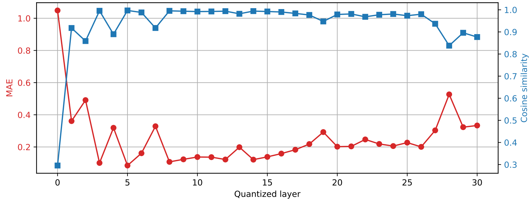
Phi-3-mini-4k-instruct | Prompt 0 Final RMSNorm output damage | float16 \rightarrow int2
