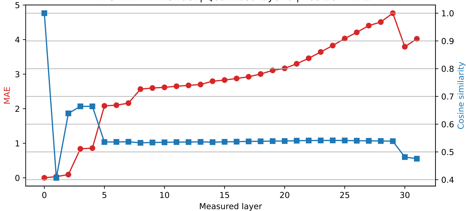
Phi-3-mini-4k-instruct | Quantized layer 0 | float16 \rightarrow int2
