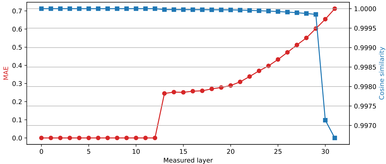
Phi-3-mini-4k-instruct | Quantized layer 12 | float16 \rightarrow int2
