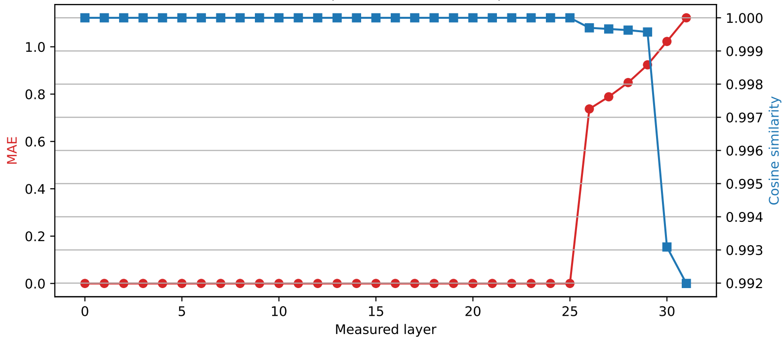
Phi-3-mini-4k-instruct | Quantized layer 25 | float16 \rightarrow int2
