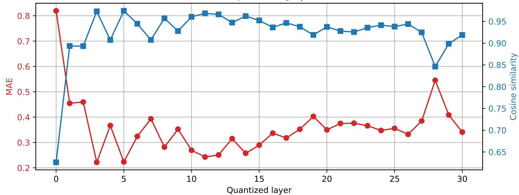
Phi-3-mini-4k-instruct | Prompt 1 Final RMSNorm output damage | float16 \rightarrow int2
