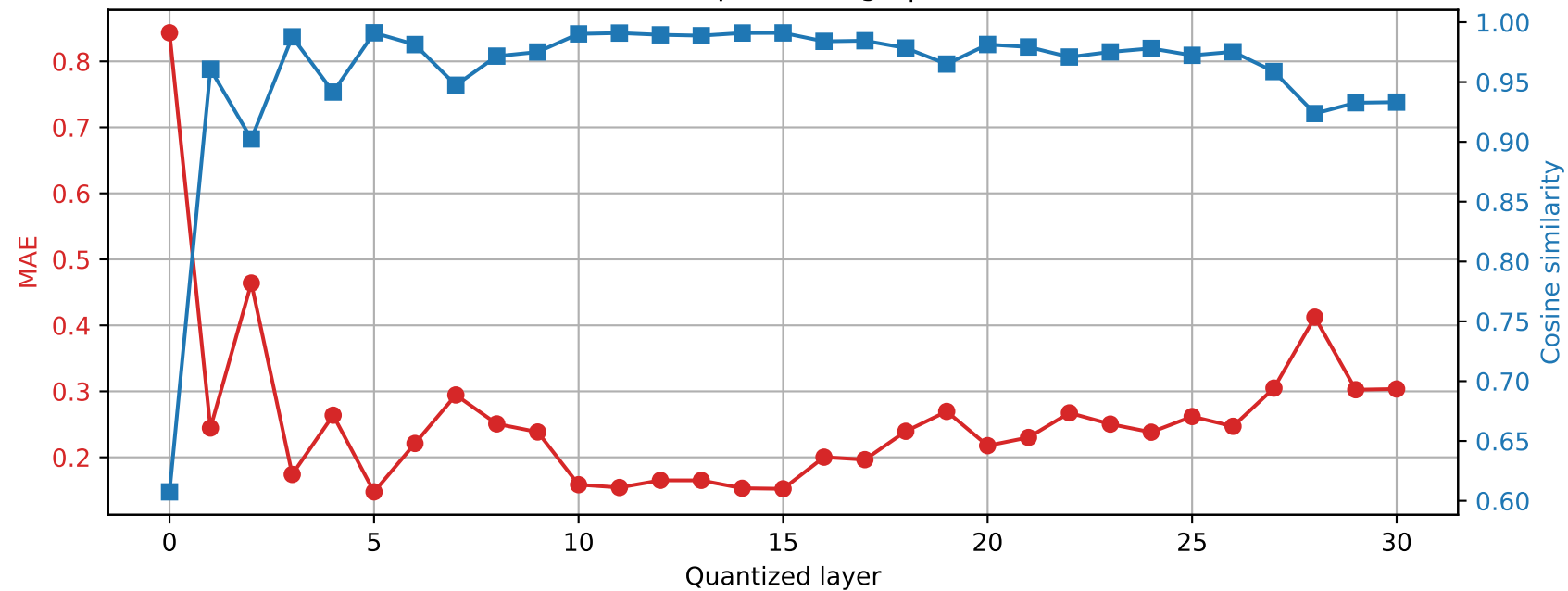
Phi-3-mini-4k-instruct | Prompt 2 Final RMSNorm output damage | float16 \rightarrow int2
