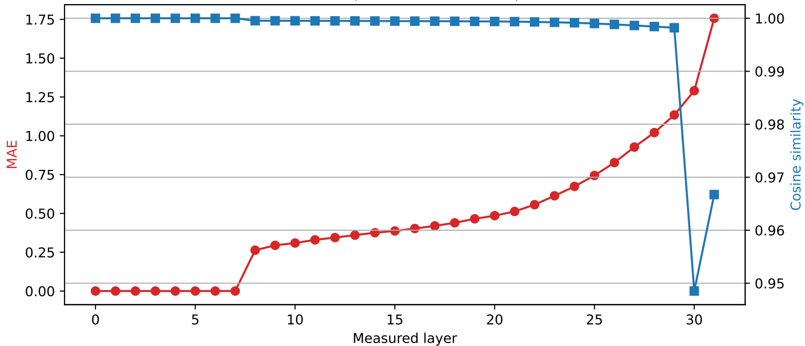
Phi-3-mini-4k-instruct | Quantized layer 7 | float16 \rightarrow int2
