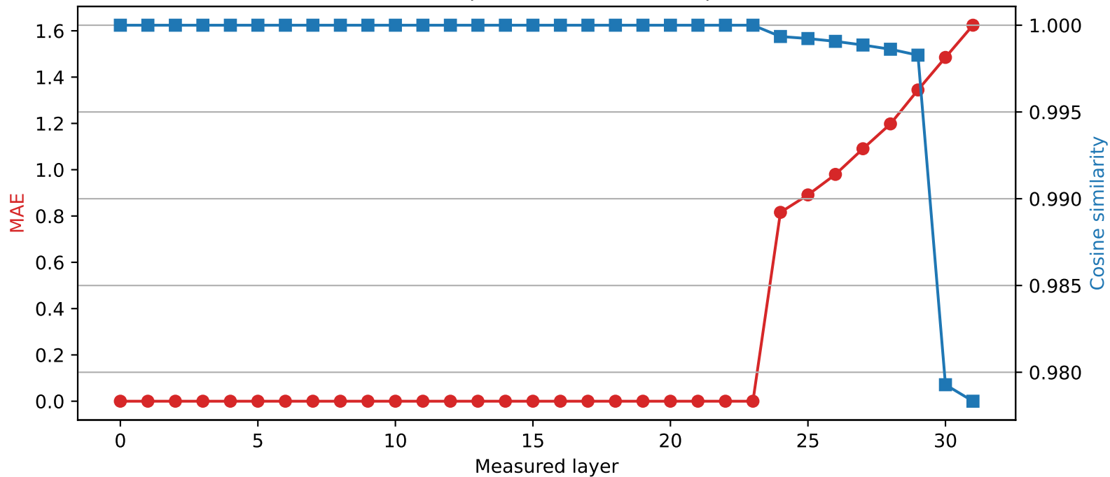
Phi-3-mini-4k-instruct | Quantized layer 23 | float16 \rightarrow int2
