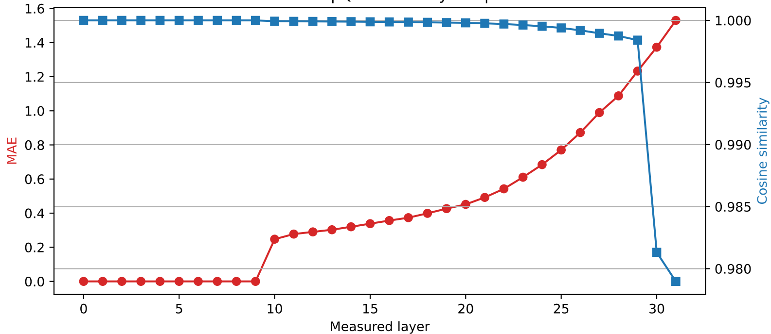
Phi-3-mini-4k-instruct | Quantized layer 9 | float16 \rightarrow int2
