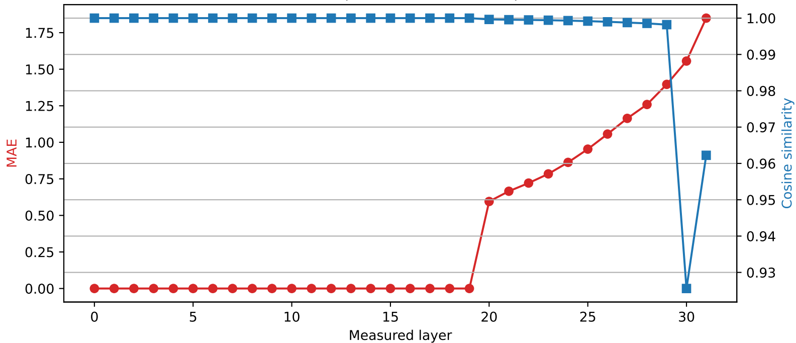
Phi-3-mini-4k-instruct | Quantized layer 19 | float16 \rightarrow int2
