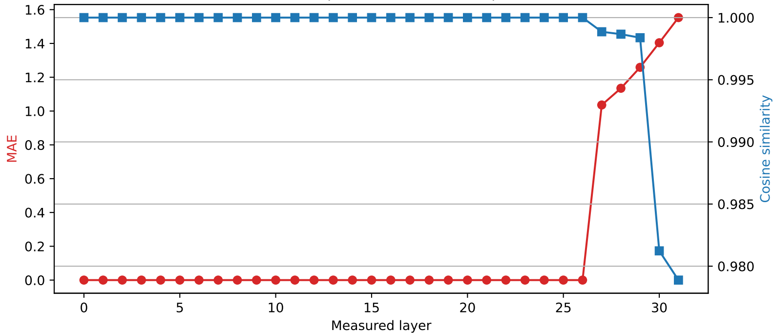
Phi-3-mini-4k-instruct | Quantized layer 26 | float16 \rightarrow int2
