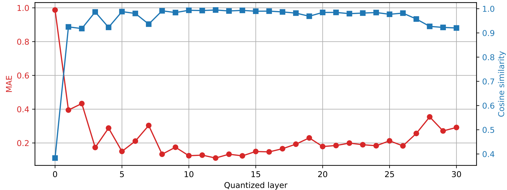
Phi-3-mini-4k-instruct | Prompt 4 Final RMSNorm output damage | float16 \rightarrow int2
