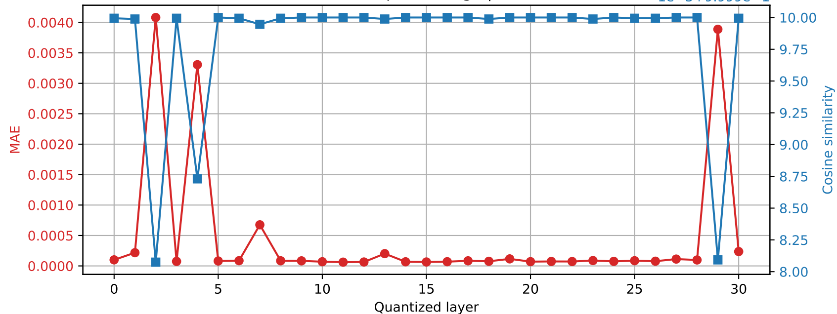
Phi-3-mini-4k-instruct | Prompt 0 Final RMSNorm output damage | float32 \rightarrow int16
