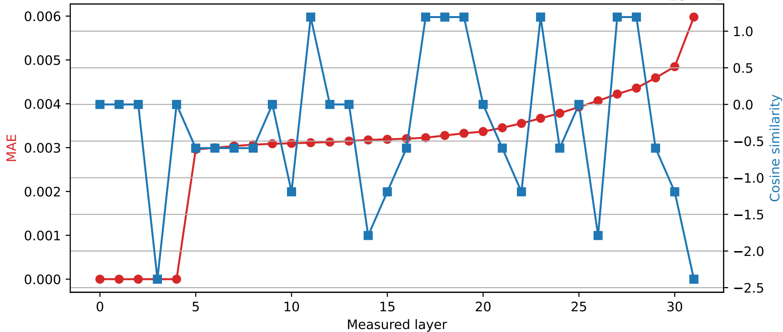
Phi-3-mini-4k-instruct | Quantized layer 4 | float32 \rightarrow int16
