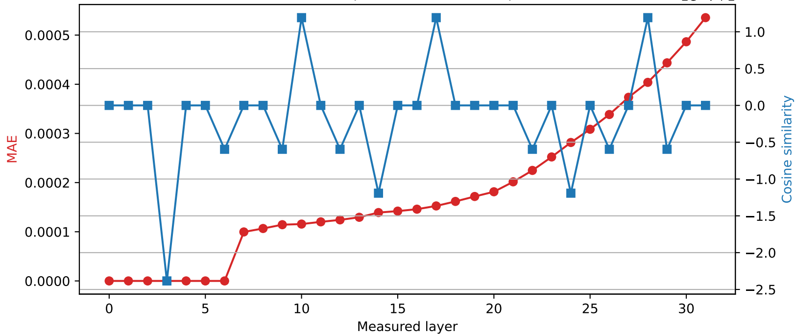
Phi-3-mini-4k-instruct | Quantized layer 6 | float32 → int16
