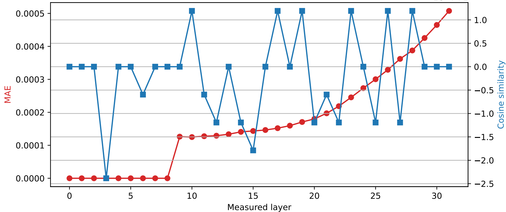
Phi-3-mini-4k-instruct | Quantized layer 8 | float32 → int16
