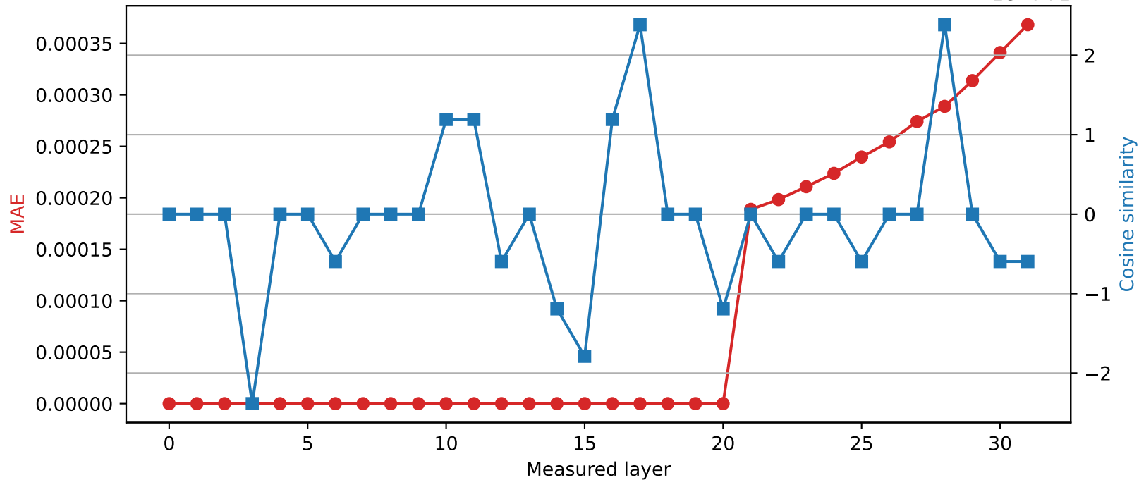
Phi-3-mini-4k-instruct | Quantized layer 20 | float32 \rightarrow int16
