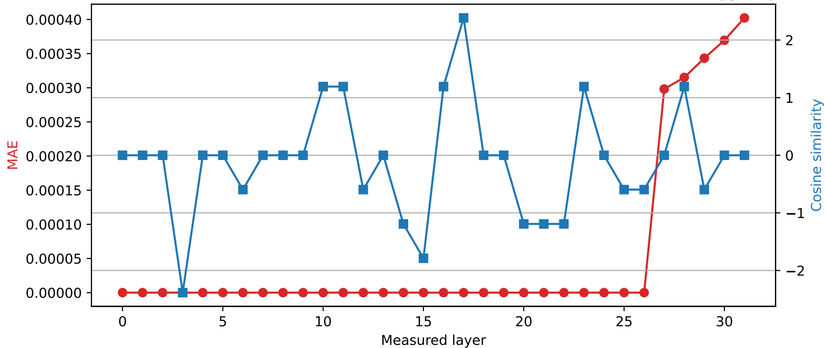
Phi-3-mini-4k-instruct | Quantized layer 26 | float32 \rightarrow int16
