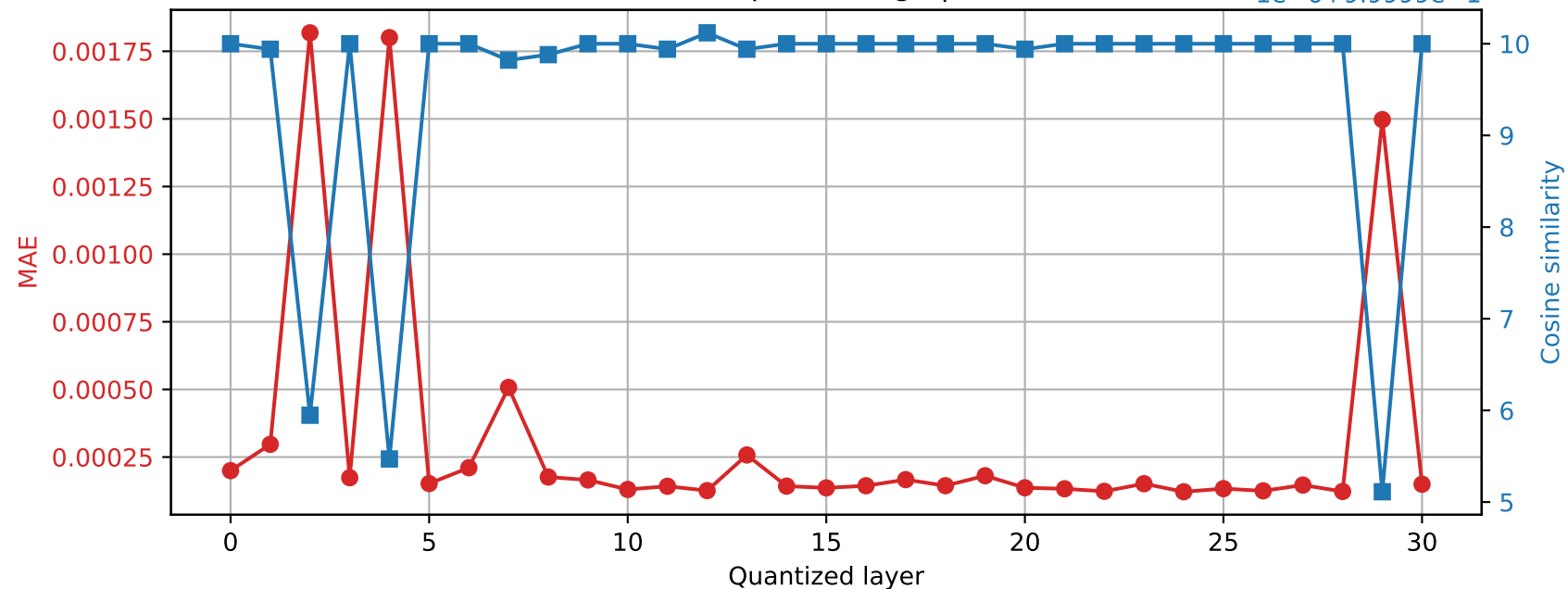
Phi-3-mini-4k-instruct | Prompt 1 Final RMSNorm output damage | float32 \rightarrow int16
