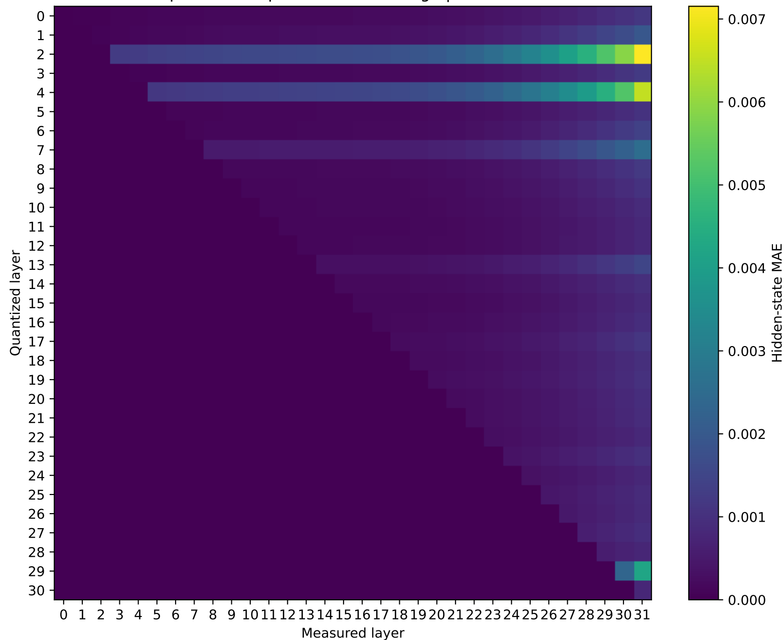
Phi-3-mini-4k-instruct Prompt 1: MAE representation damage | float32 \rightarrow int16
