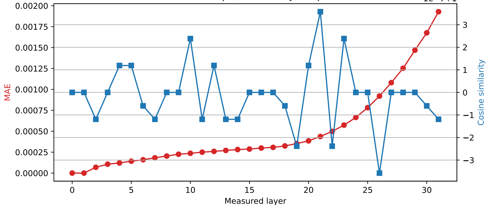
Phi-3-mini-4k-instruct | Quantized layer 1 | float32 \rightarrow int16
