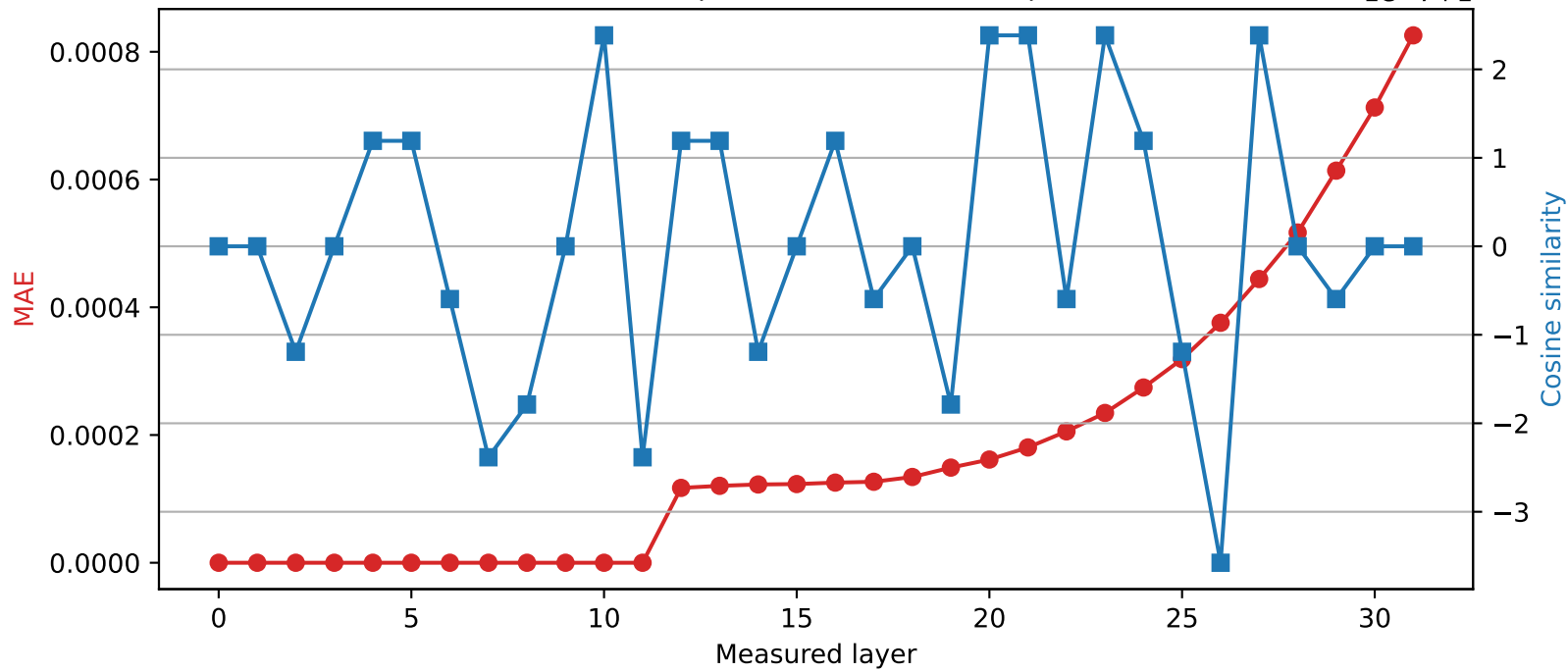
Phi-3-mini-4k-instruct | Quantized layer 11 | float32 \rightarrow int16
