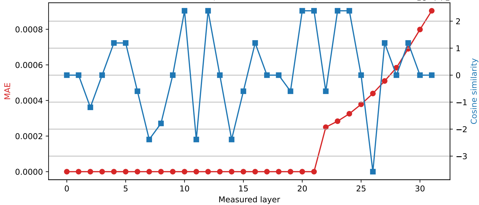
Phi-3-mini-4k-instruct | Quantized layer 21 | float32 \rightarrow int16
