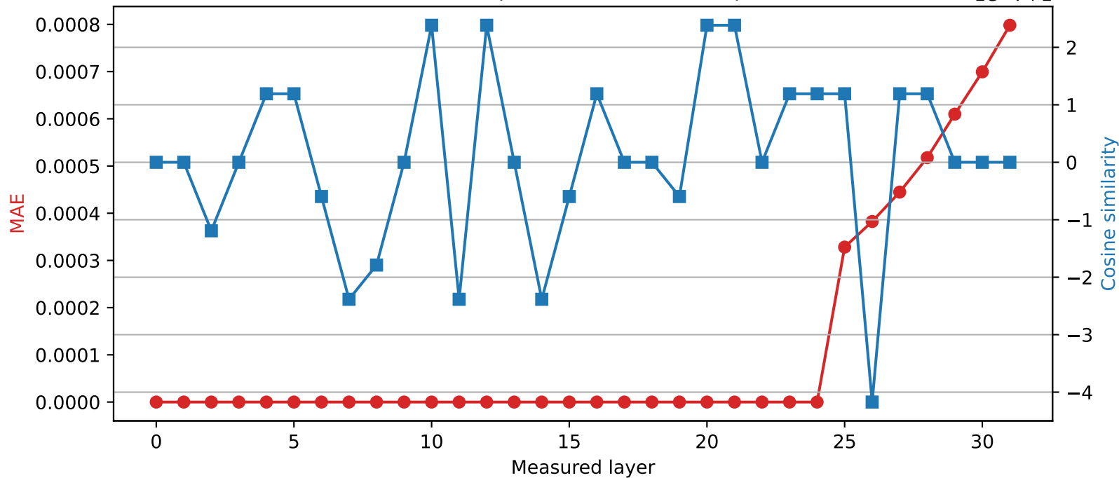
Phi-3-mini-4k-instruct | Quantized layer 24 | float32 \rightarrow int16
