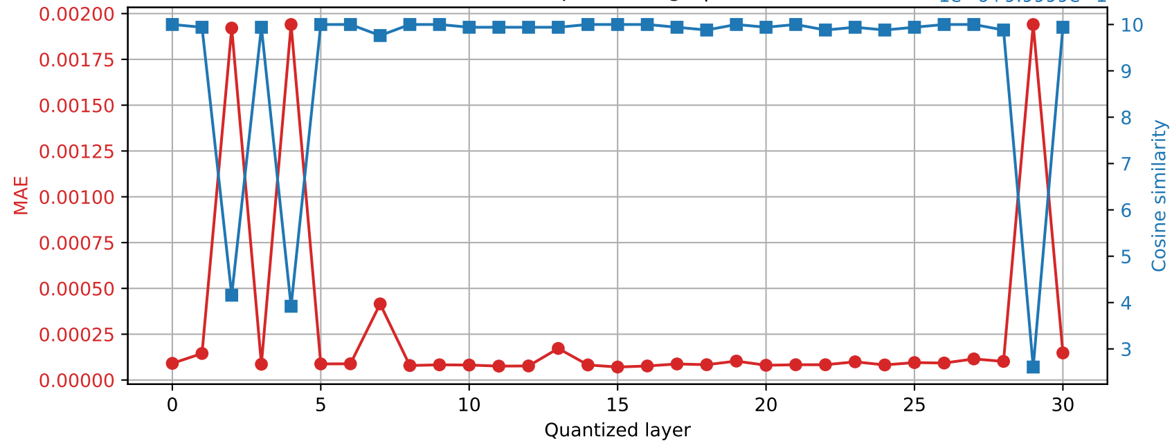
Phi-3-mini-4k-instruct | Prompt 2 Final RMSNorm output damage | float32 \rightarrow int16
