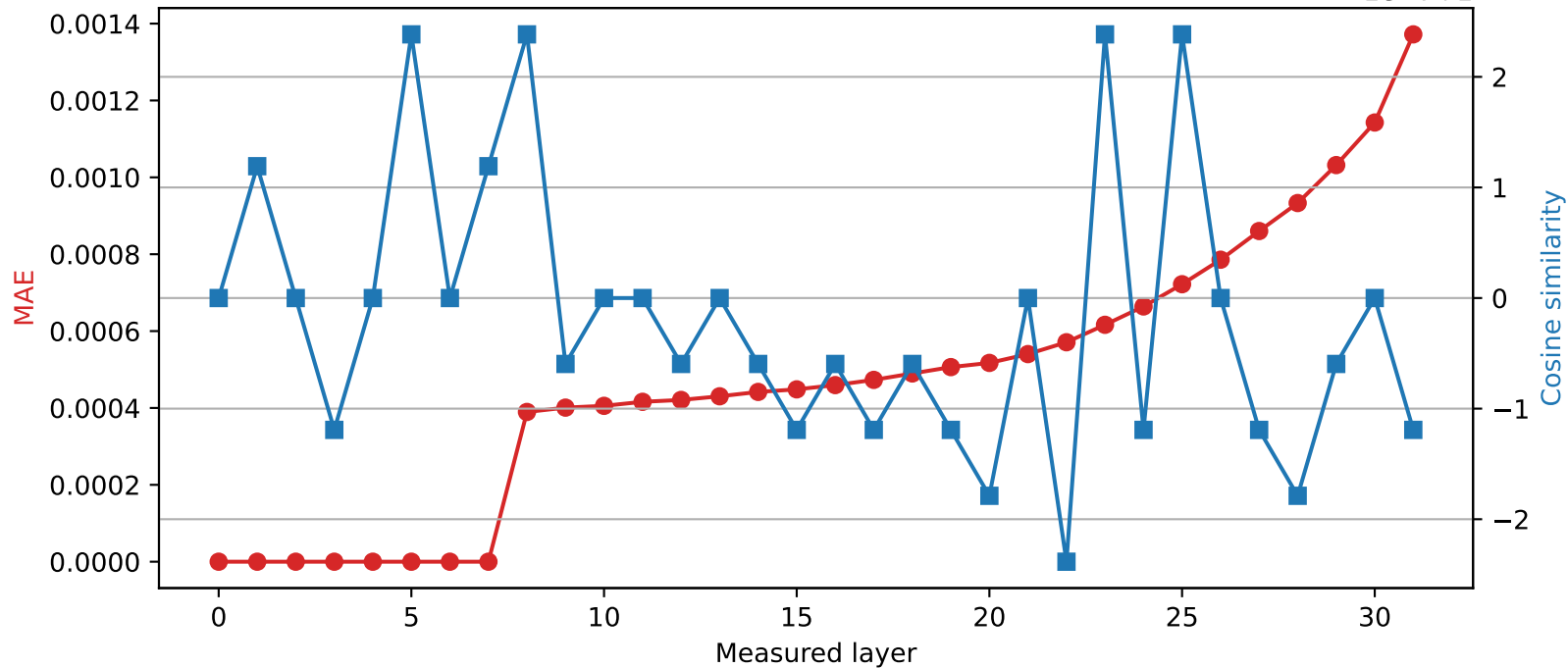
Phi-3-mini-4k-instruct | Quantized layer 7 | float32 → int16
