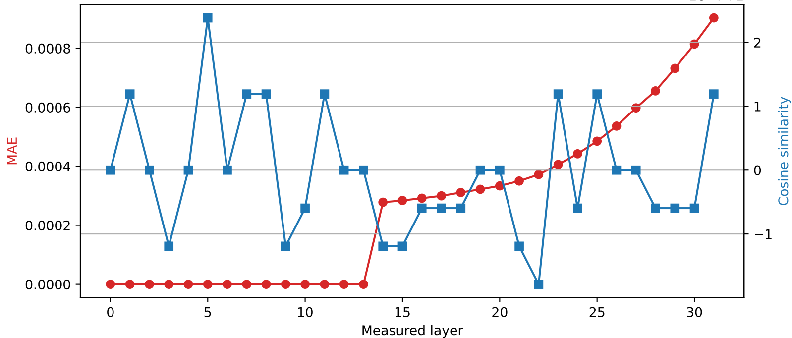
Phi-3-mini-4k-instruct | Quantized layer 13 | float32 \rightarrow int16
