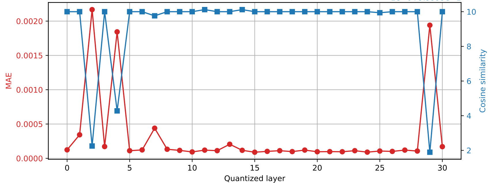
Phi-3-mini-4k-instruct | Prompt 3 Final RMSNorm output damage | float32 \rightarrow int16
