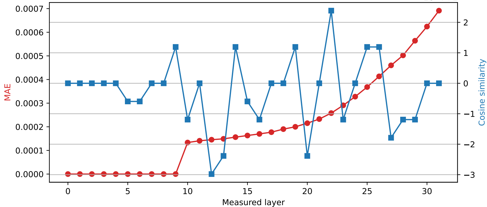
Phi-3-mini-4k-instruct | Quantized layer 9 | float32 \rightarrow int16
