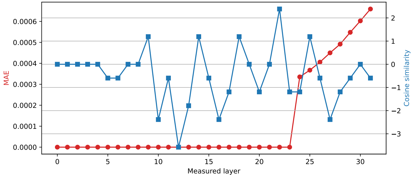
Phi-3-mini-4k-instruct | Quantized layer 23 | float32 \rightarrow int16
