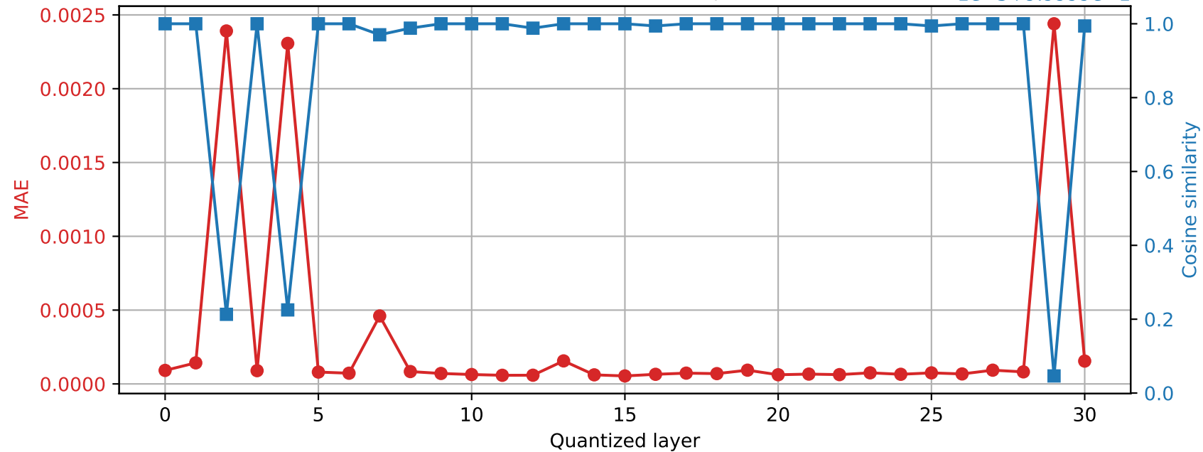
Phi-3-mini-4k-instruct | Prompt 4 Final RMSNorm output damage | float32 \rightarrow int16
