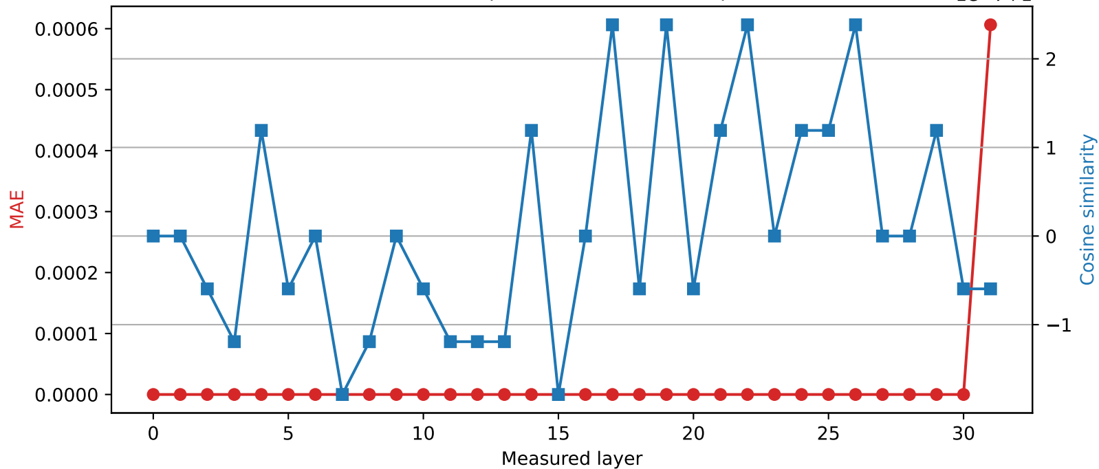
Phi-3-mini-4k-instruct | Quantized layer 30 | float32 \rightarrow int16
