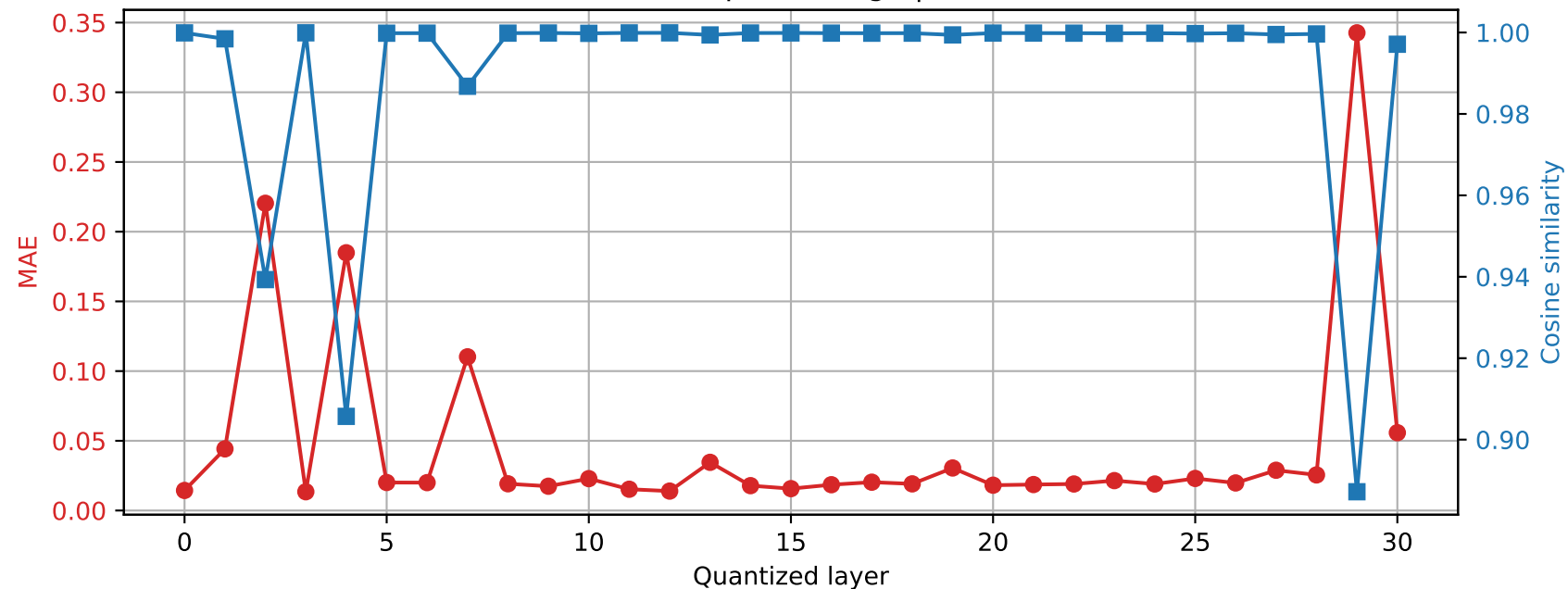
Phi-3-mini-4k-instruct | Prompt 0 Final RMSNorm output damage | float32 \rightarrow int8
