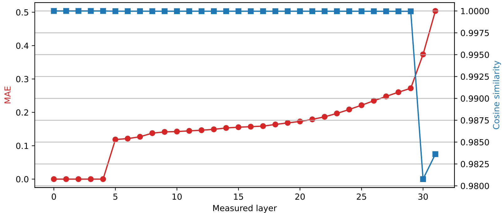
Phi-3-mini-4k-instruct | Quantized layer 4 | float32 \rightarrow int8
