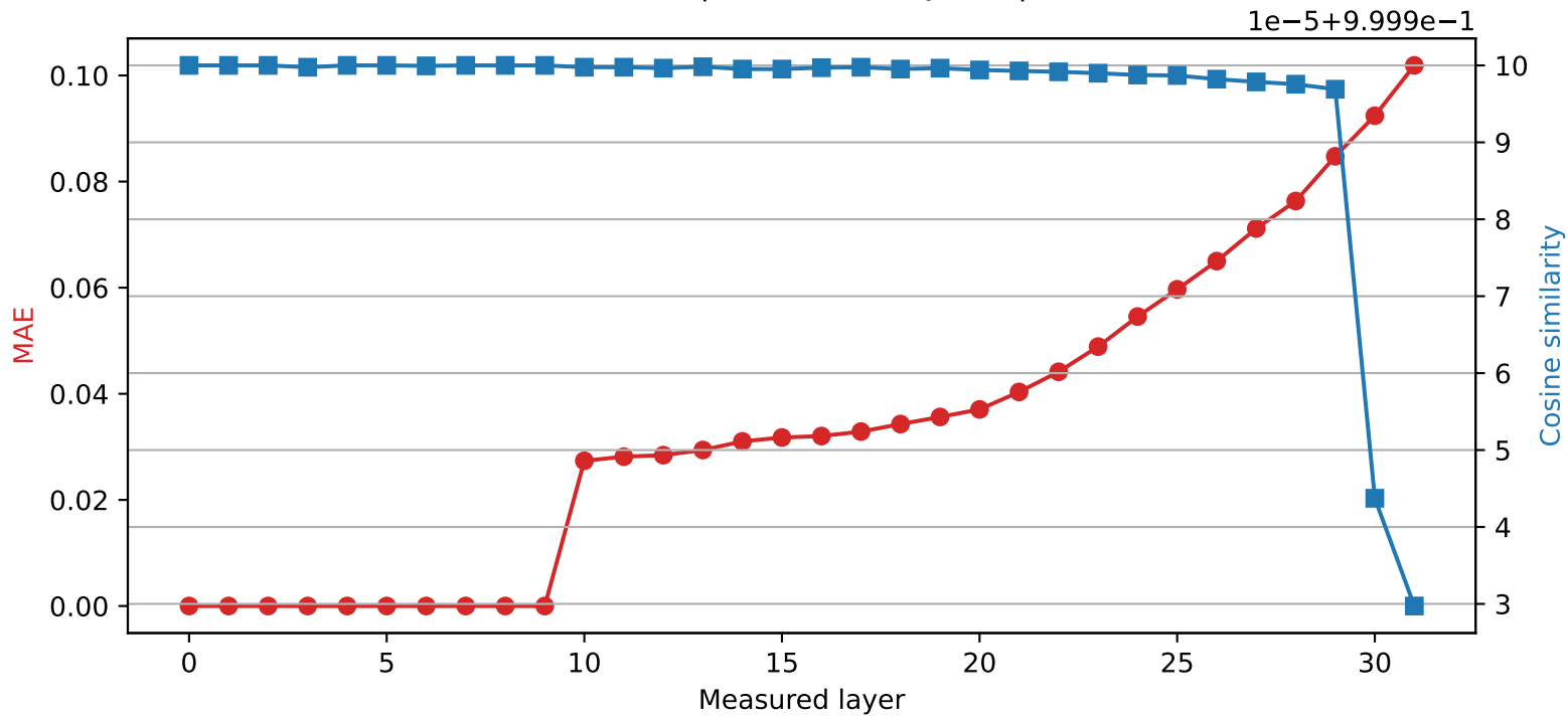
Phi-3-mini-4k-instruct | Quantized layer 9 | float32 → int8
