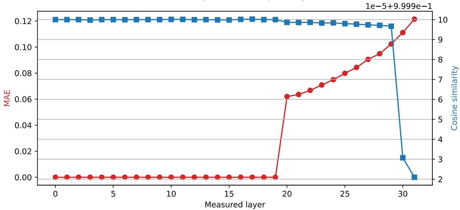
Phi-3-mini-4k-instruct | Quantized layer 19 | float32 → int8
