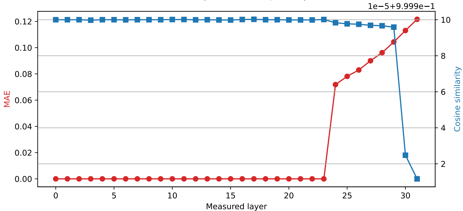
Phi-3-mini-4k-instruct | Quantized layer 23 | float32 \rightarrow int8
